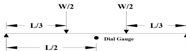
Fig 9. Two-point loading setup
