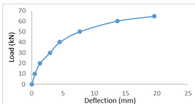
Graph.5: Load Vs Deflection graph for rectangular opening equivalent to hexagonal 45° opening
