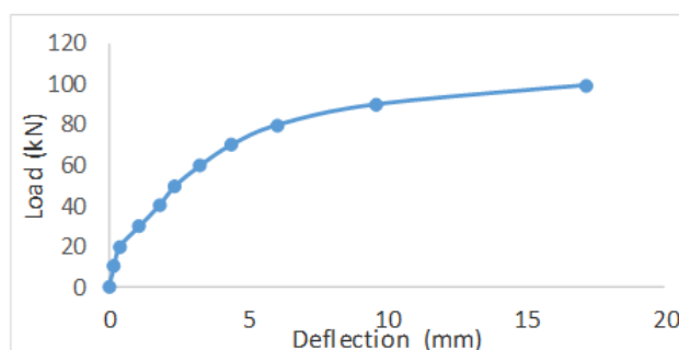
Graph.6: Load Vs Deflection graph for rectangular opening equivalent to hexagonal 60° openings.
