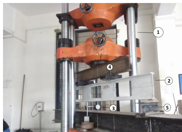
Fig 9. Two-point loading setup
