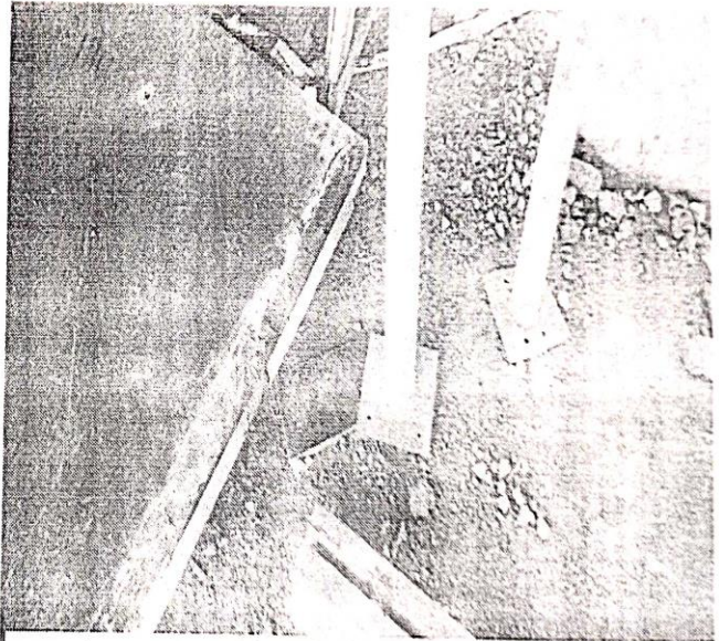
Baseplate fixity in props needs perfection observed defective
