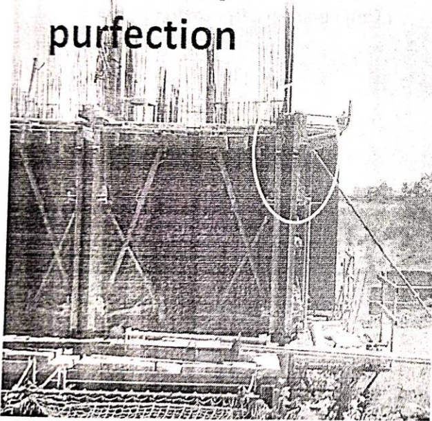
Baseplate fixity in props needs perfection observed defective
