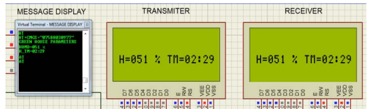
Fig. 8. Simulated Results for Humidity > 45%.
