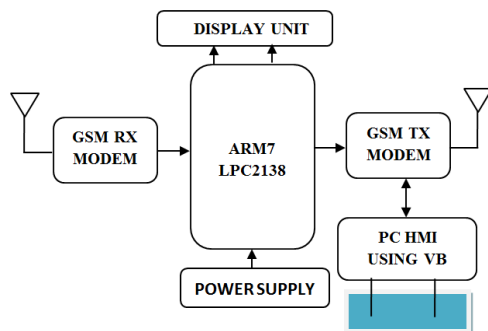
Fig.2. Block diagram of control section of proposed system.
