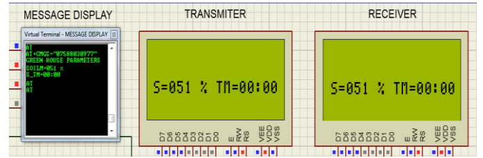
Fig. 12. Simulated results of airflow with anemometer RPM > 50.
