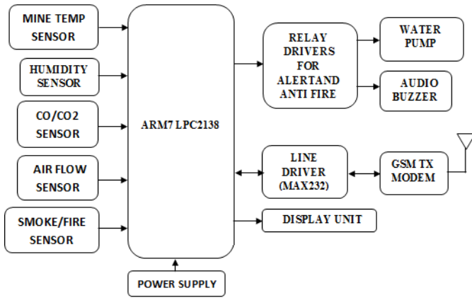
Fig. 1. Block diagram of sensor section of proposed system.
