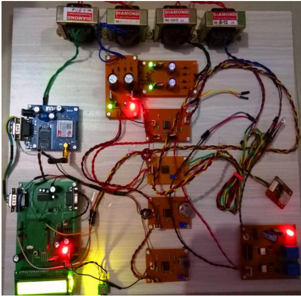
Fig.16. Photograph of fabricated project for GSM Operated Wireless Sensor Based Mine Security and Safety.
