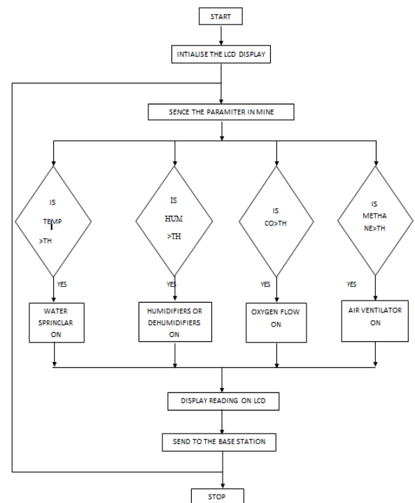
Fig. 3. flow chart for sensor section.
