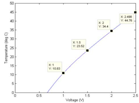
Fig. 6. Temperature sensor voltage relationship.
