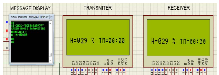
Fig. 7. Simulated result for humidity < 45%.
