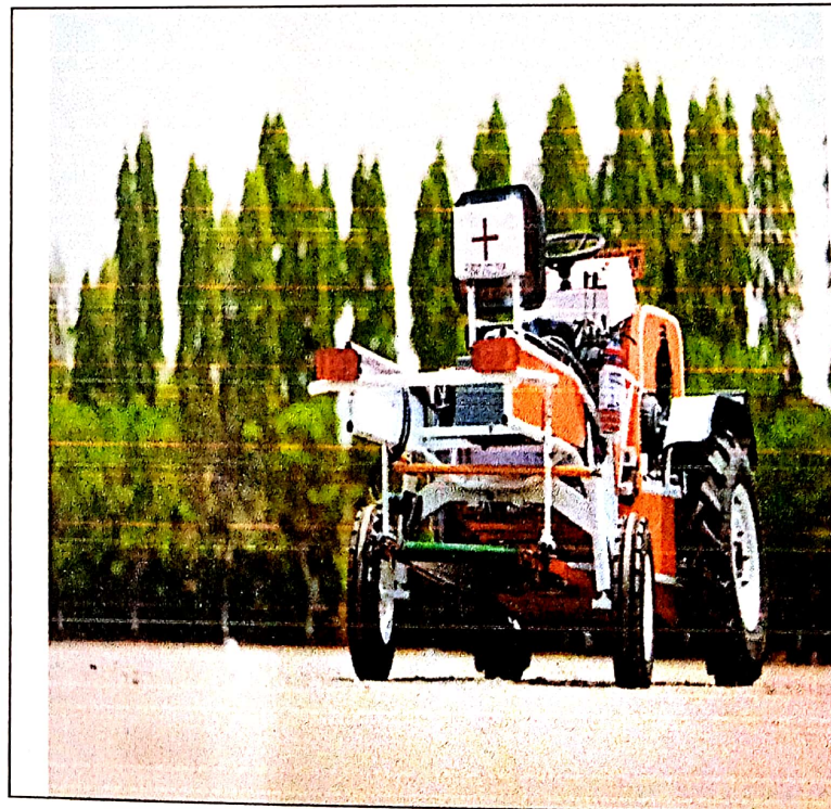
Figure 11.1 Self-Propelled Onion Harvester
