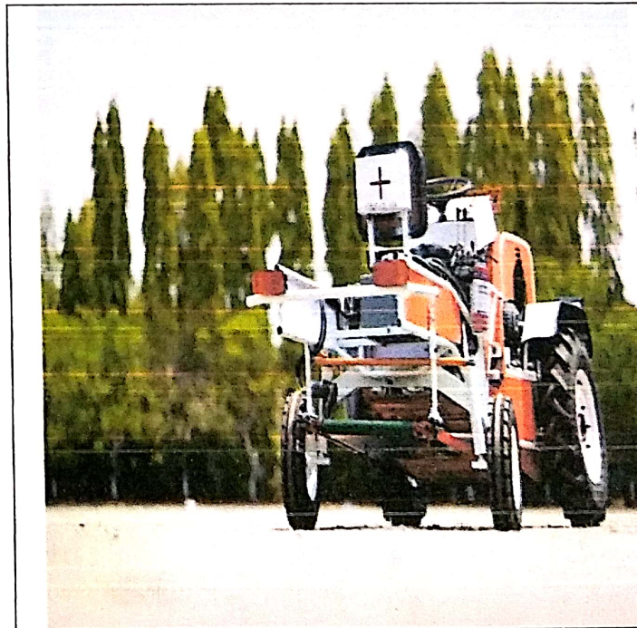
Figure 11.1 Self-Propelled Onion Harvester
