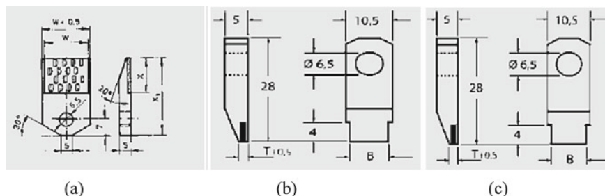
Fig. 6.1 Types of multi-point dressers. a Needle blade with natural diamond dresser, b MCD needle blade dresser, c CVD needle blade dresser [1]
