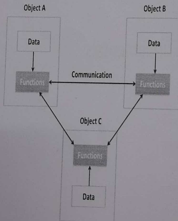
Organization of data & functions in OOP
