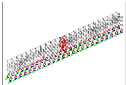
Fig. 5. Geometry of pipe rack with bracings at center
